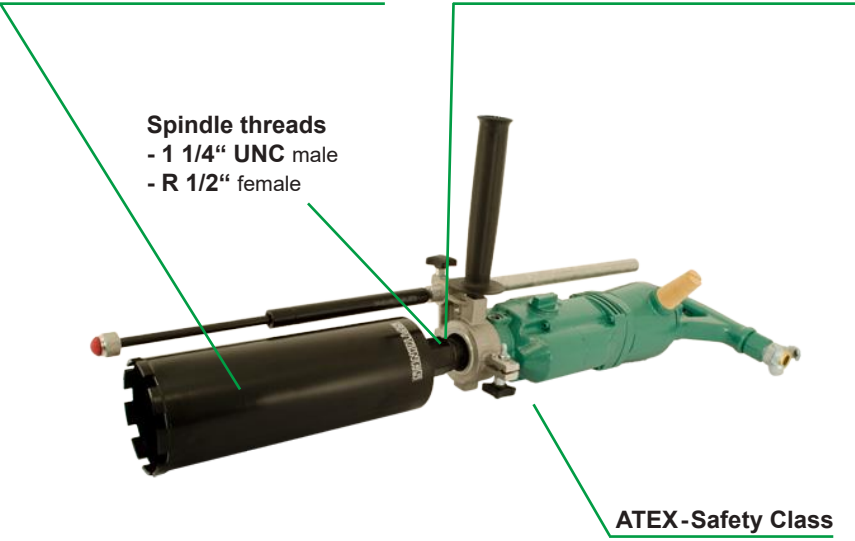
Drill bit adapter and water connection
