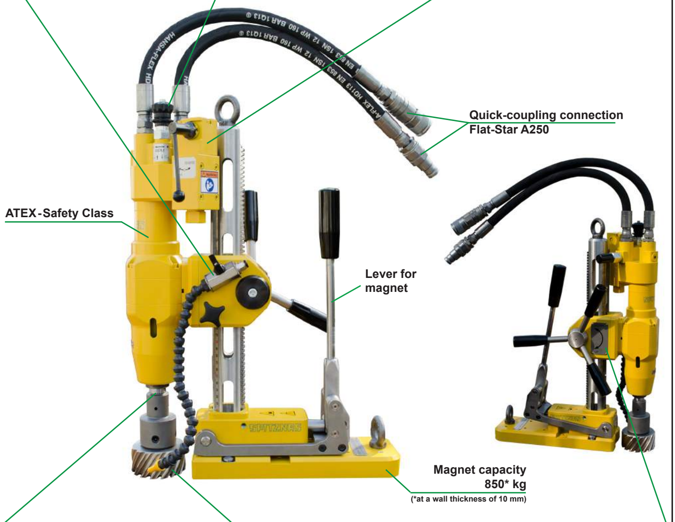
Tool holder MT3
